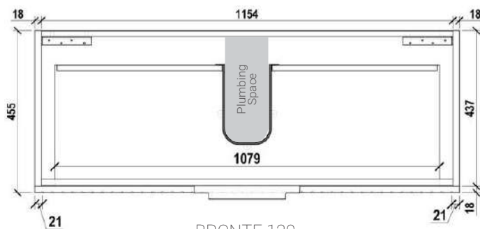
BRONTE 120 Top Section
