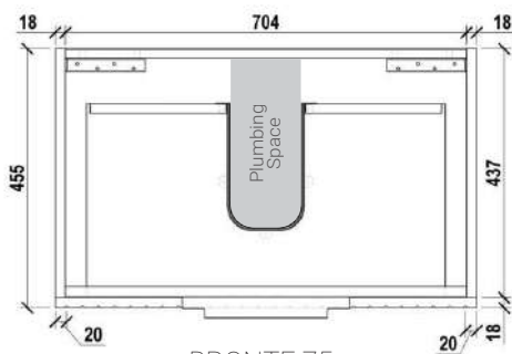
BRONTE 75 Top Section
