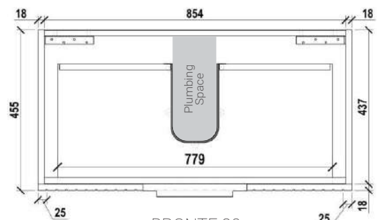
BRONTE 90 Top Section
