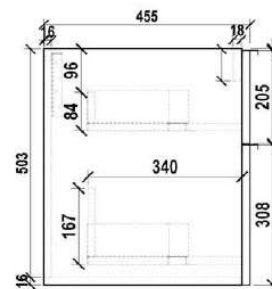
ALL SIZES Side Section
