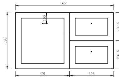
AUSTIN90WH Front View
