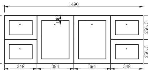
AUSTIN150WH Front View
