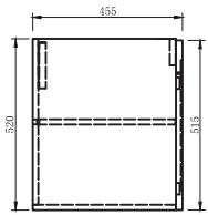
AUSTIN60WH Side Section
