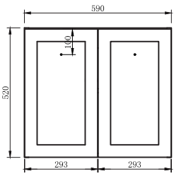
AUSTIN60WH Front View
