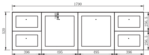
AUSTIN180WH Front View
