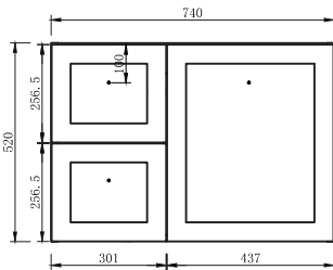
AUSTIN75WH Front View
