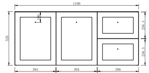
AUSTIN120WH Front View
